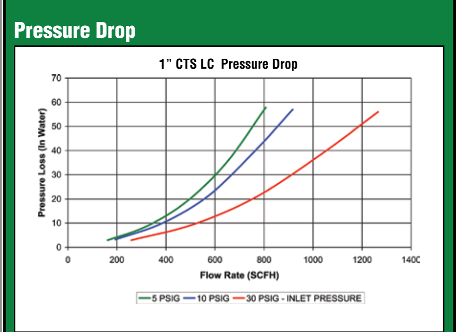
18" Water Column Pressure Drop at Maximum Trip Flow Rate
