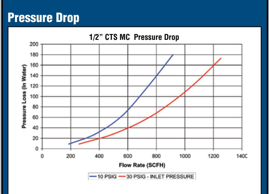
348" Water Column Pressure Drop at Maximum Trip Flow Rate
